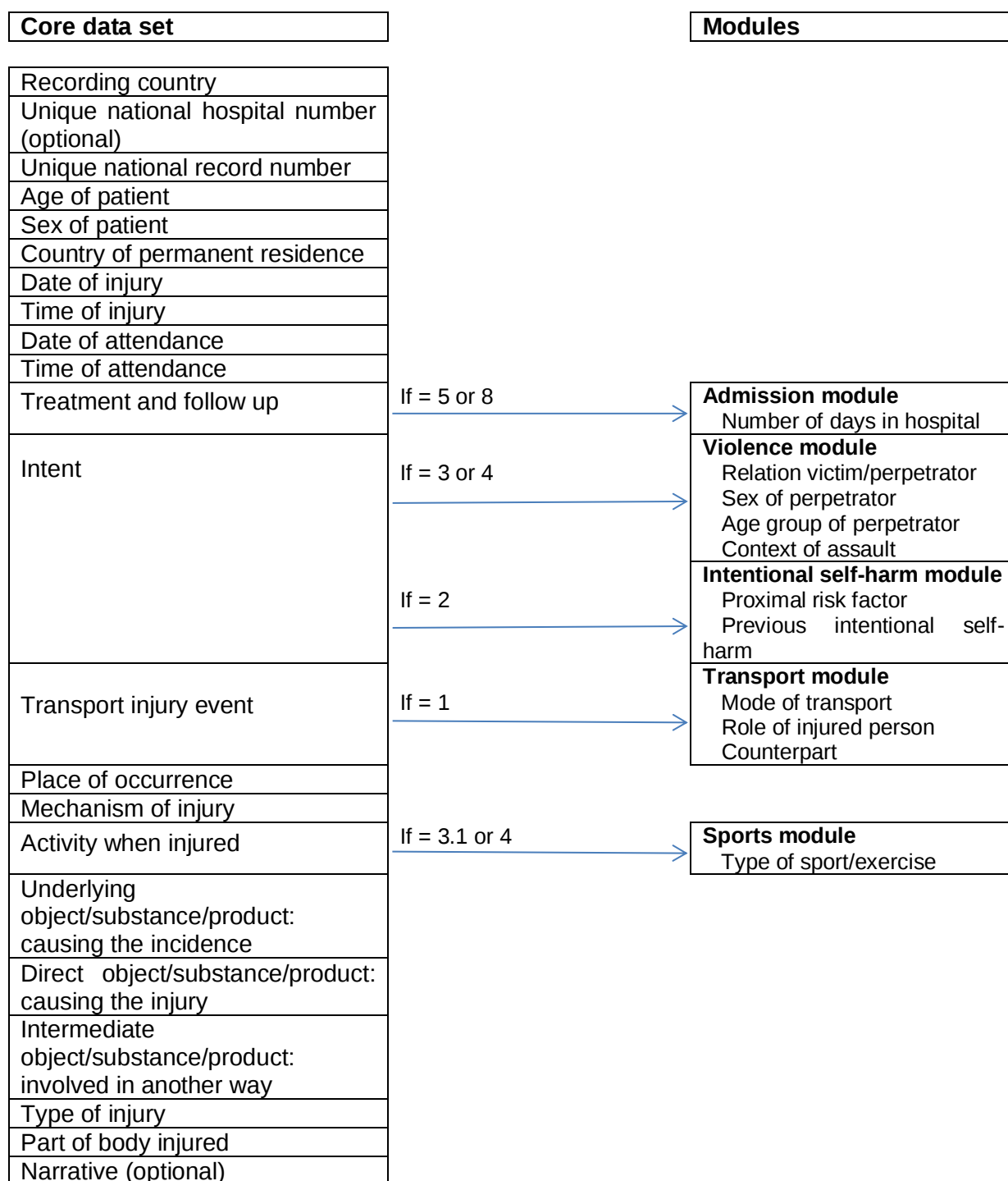
Figure 1: Data elements of the core set of the IDB-FDS and guideline for using the modules
